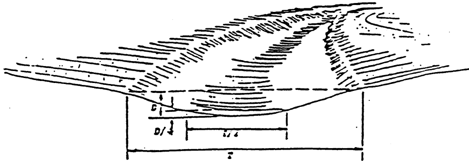
PARABOLIC CROSS-SECTION
