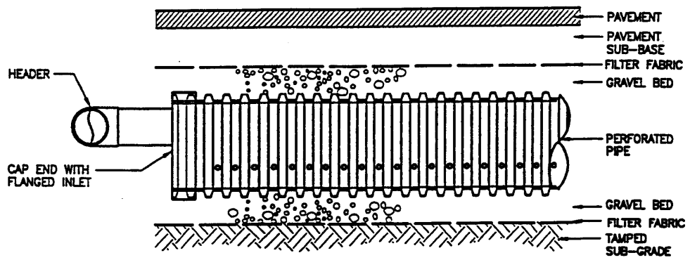
ALTERNATE CONSTRUCTION USING PERFORATED PIPE
