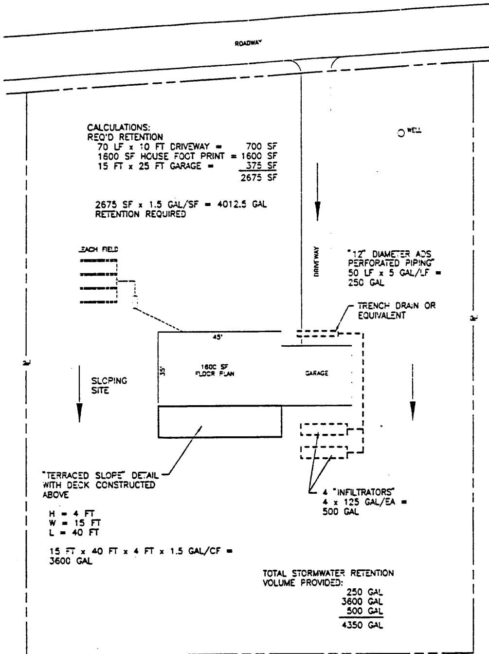
FIGURE 6-2 EXAMPLE SITE #2 SLOPING SITE
