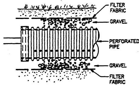
USE OF CONSTRUCTION TRENCH
