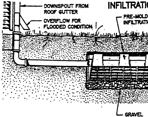
USE OF PREMOLDED INFILTRATION UNIT
