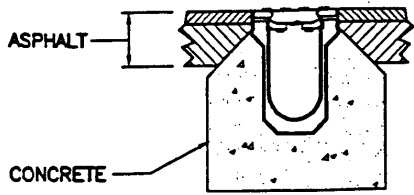
ASPHALT INSTALLATION
