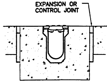
CONCRETE INSTALLATION
